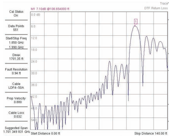
Picture 14: DTF with TMA in path
