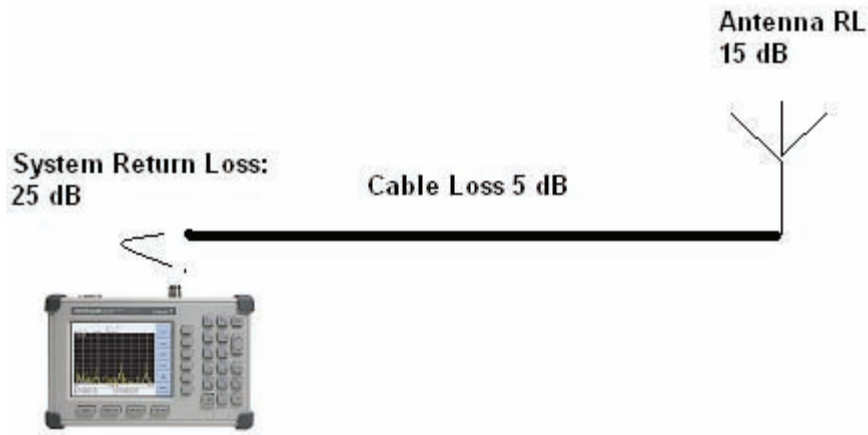
Picture 4: System Return Loss setup
